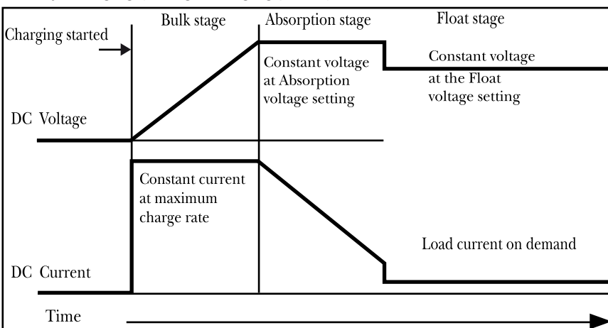
Battery Charging (3 stage charging profile)
